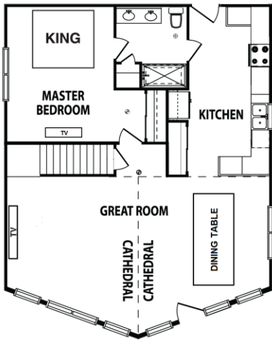
Main Level
